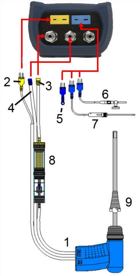
Fig. 1: Connection diagram (Sensor side)
