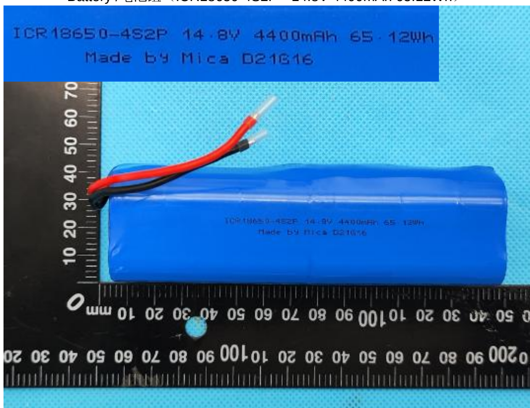
Battery /电池组 (ICR18650-4S2P 14.8V 4400mAh 65.12Wh)
