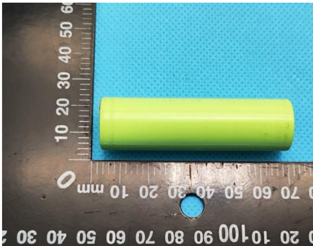
Cell /电芯 (ICR18650 3.7V 2200mAh 8.14Wh)
