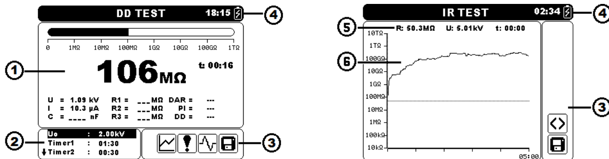
Figure 3.4: Typical function display and graph screen
