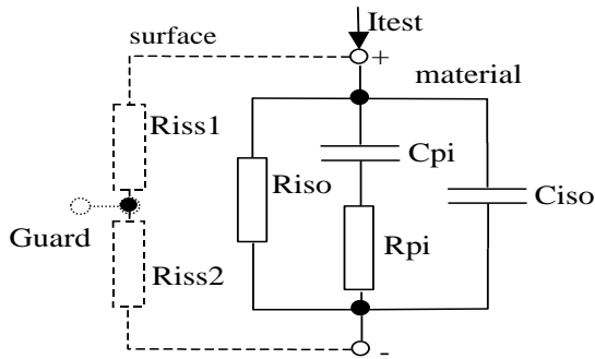
Figure 5.1: Insulating material
