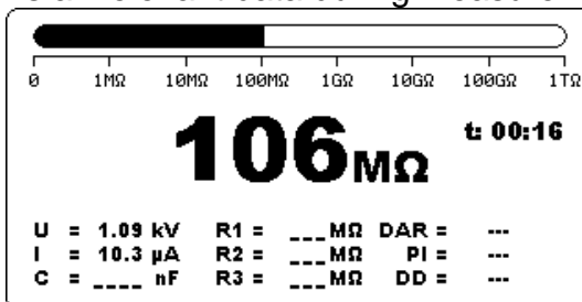
Figure 3.5: Measurement window
