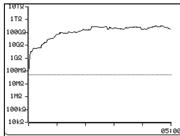
Figure 3.8: Graph screen
