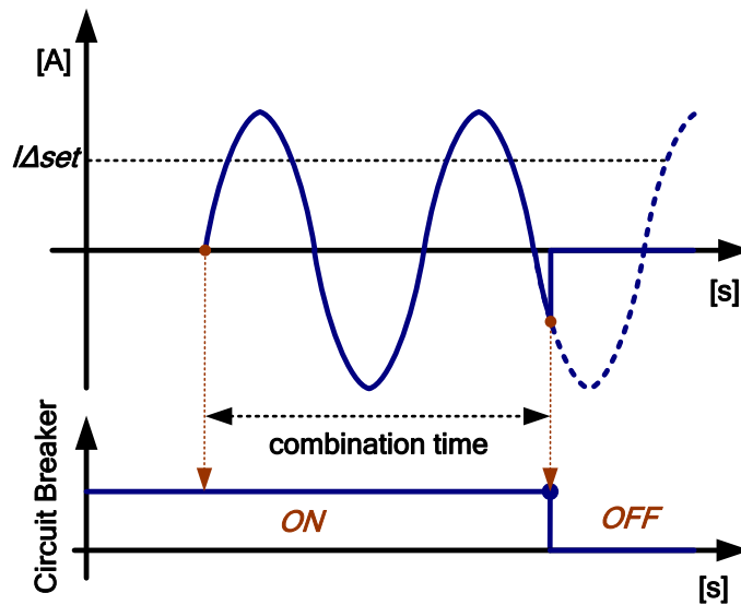
Figure 6.20: ELR Combination Time Test current waveforms example
