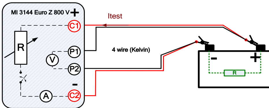
Figure 6.10: R line mΩ Measurement example 1 (battery)
