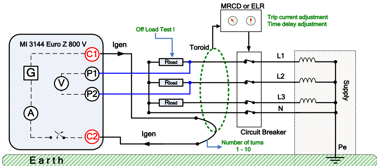
Figure 6.16: ELR Current Injection Test and Combination Time Test example
