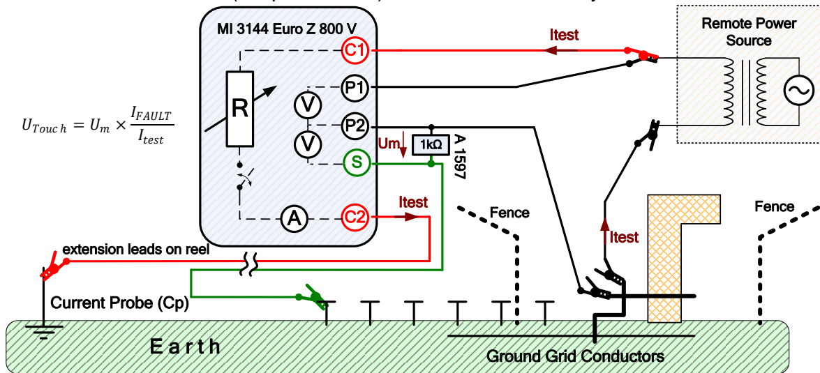
Figure 6.14: U touch Measurement example
